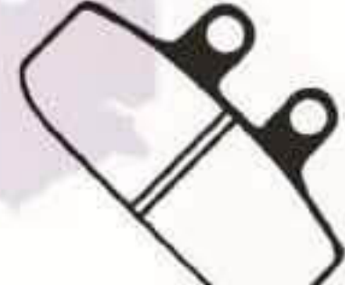
OH101 71x36.3x9.2mm BX16061028 YAMAHA DT125
